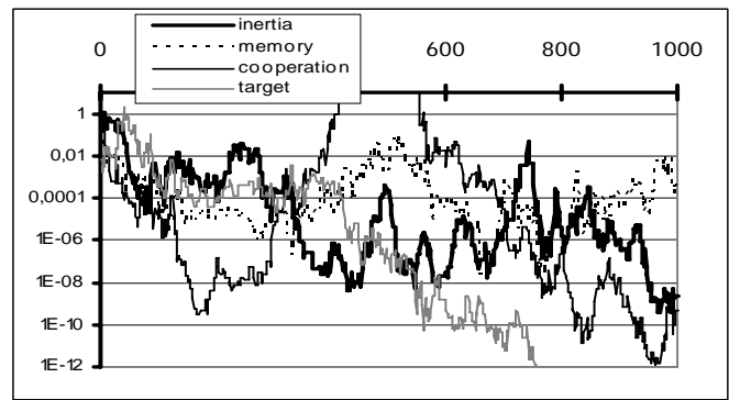
Figure 5 – Evolution of weights of a particle during the unit commitment optimization (1000 generations) using dEPSO.
