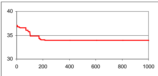
Figure 4 – Evolution of the best fitness during 1000 generations in one run of the dEPSO algorithm
