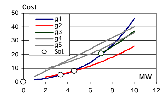
Figure 1 – Cost curves for the unit commitment problem and the best solution with 3 generators dispatched and 2 shut down.
